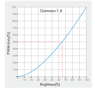
Dimming curve for RGBW/RGB/DIM
